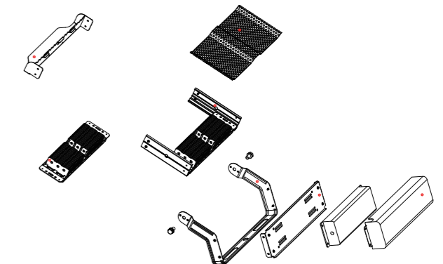
Explosion structure
